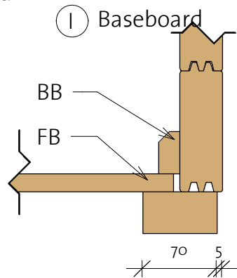
Floor Schedule
